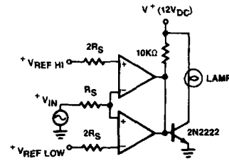
Limit Comparator
