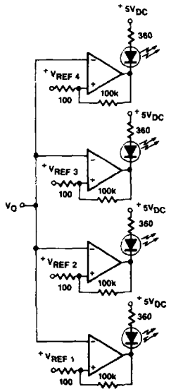
Visible Voltage Indicator
