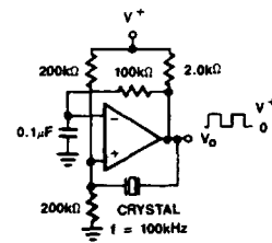
Crystal-Controlled Oscillator
