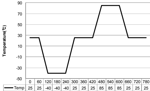
Temperature Cycle
