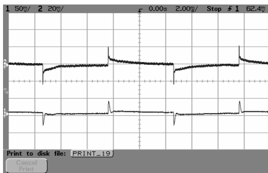
ALQ07FM 25%-50%-25% I_{o2,nom} ( I_{o2} ) load change, I_{o1} = 50\%I_{o1,nom} (ch1: V_{o1} ,ch2: V_{o2} )
