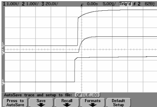
ALQ07FY Start-up from Power On
