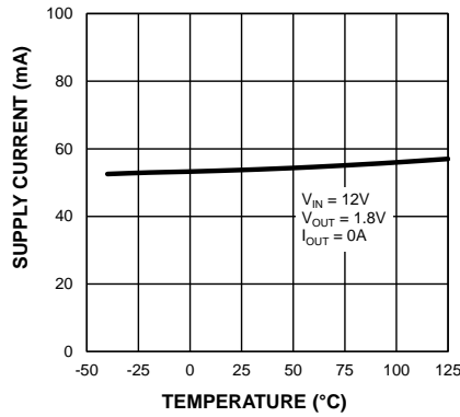
VIN Operating Supply Current vs. Temperature (MIC45212-2)
