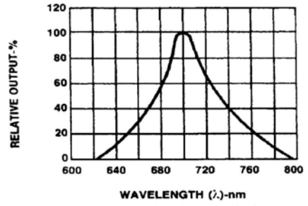
Fig.2 SPECTRAL RESPONSE
