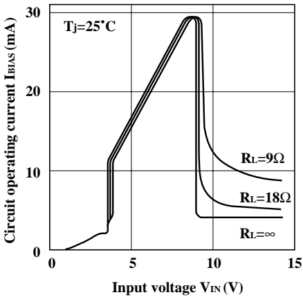
Fig.19 Circuit Operating Current vs. Input Voltage (PQ12SZ1/PQ12SZ11)
