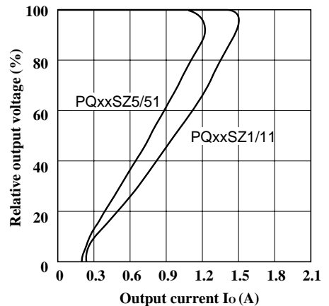
Fig.3 Overcurrent Protection Characteristics(Typical Value)
