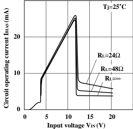
Fig.20 Circuit Operating Current vs. Input Voltage (PQ12SZ5/PQ12SZ51)
