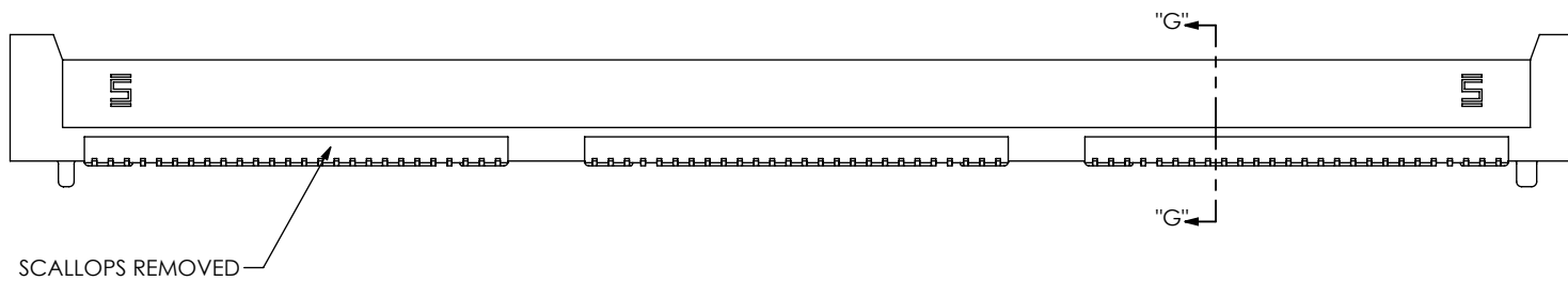
FIG 10 (QRF8-078-05.0-X-D-A SHOWN) (DIFFERENT AS SHOWN FOR ALL 3 BANK ASSEMBLIES) SCALE 4:1
