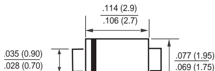
SOD-123FL
