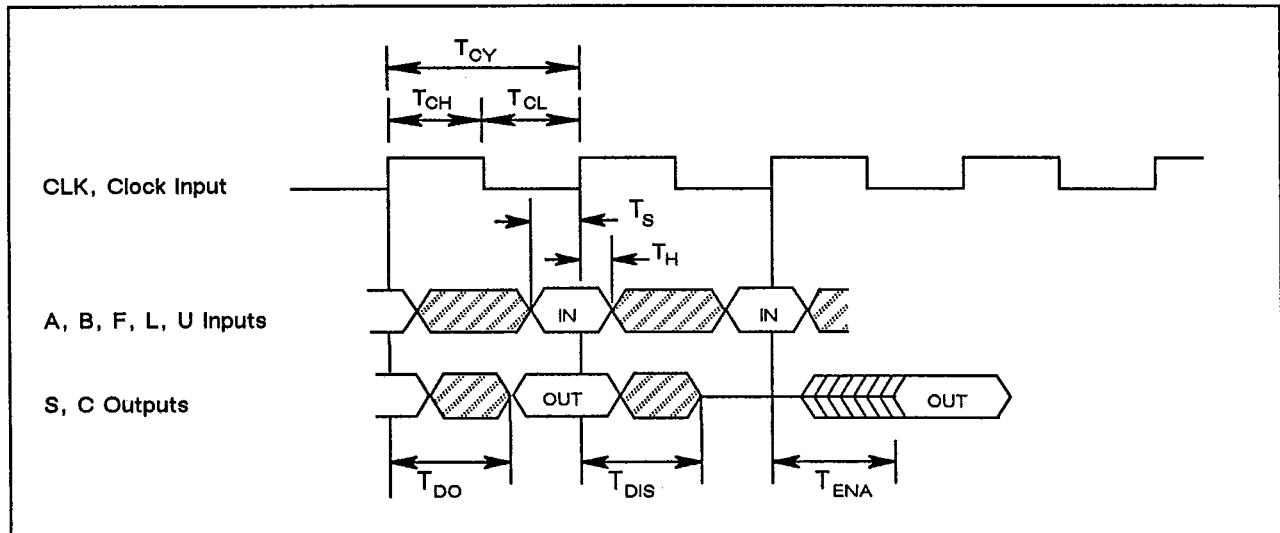
Figure 8. Switching Characteristics
