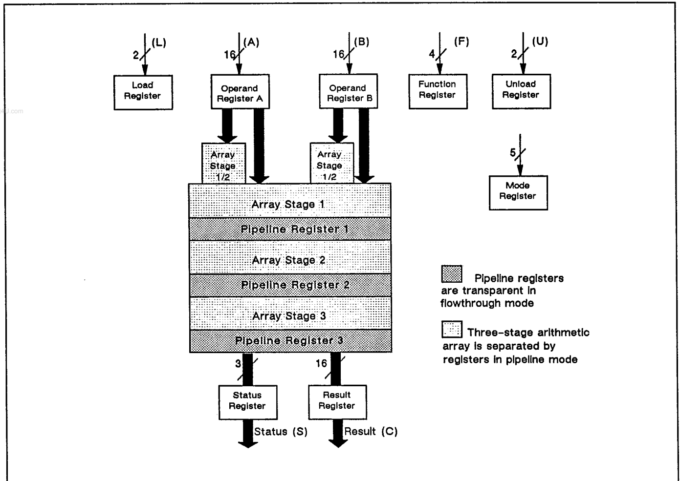
Figure 1. WTL 1232 Multiplier and 1233 ALU Data Path Architecture
