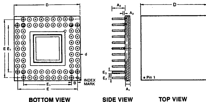
68-PIN PIN GRID ARRAY
