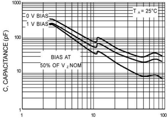
Figure 5. Typical Capacitance
