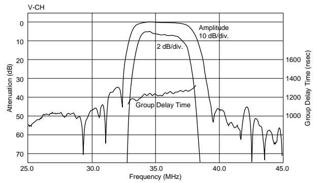
Frequency Characteristics(Pictuer-ch)
