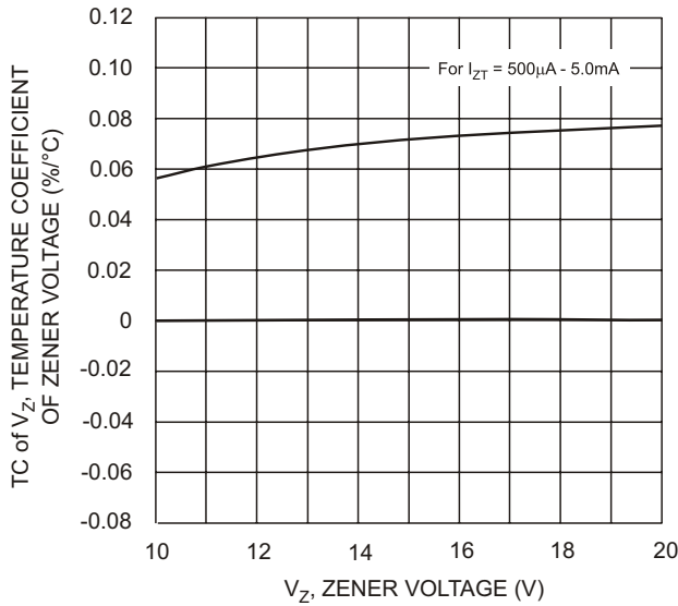
TC of V_Z , TEMPERATURE COEFFICIENT OF ZENER VOLTAGE (%/°C) For I_{ZT} = 500\mu\text{A} - 5.0\text{mA} V_Z , ZENER VOLTAGE (V) Fig. 9 Typical Temperature Coefficient of Zener Voltage vs. Zener Voltage, UDZ10B-UDZ20B
