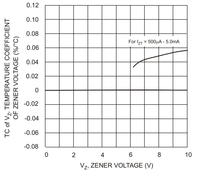
TC of V_Z , TEMPERATURE COEFFICIENT OF ZENER VOLTAGE (%/°C) For I_{ZT} = 500\mu\text{A} - 5.0\text{mA} V_Z , ZENER VOLTAGE (V) Fig. 8 Typical Temperature Coefficient of Zener Voltage vs. Zener Voltage, UDZ6V2B-UDZ10B
