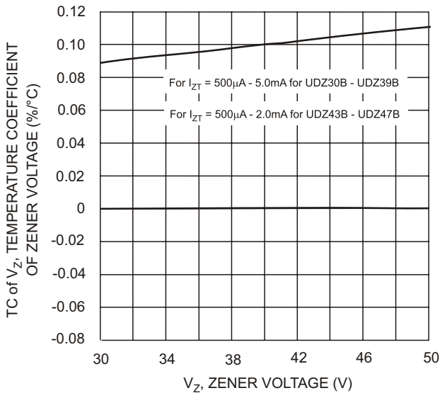
TC of V_Z , TEMPERATURE COEFFICIENT OF ZENER VOLTAGE (%/°C) For I_{ZT} = 500\mu\text{A} - 5.0\text{mA} for UDZ30B - UDZ39B For I_{ZT} = 500\mu\text{A} - 2.0\text{mA} for UDZ43B - UDZ47B V_Z , ZENER VOLTAGE (V) Fig. 11 Typical Temperature Coefficient of Zener Voltage, UDZ30B-UDZ47B
