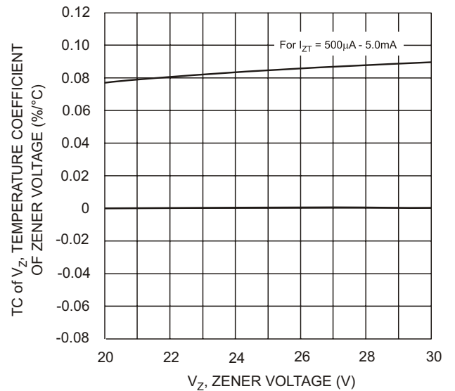
TC of V_Z , TEMPERATURE COEFFICIENT OF ZENER VOLTAGE (%/°C) For I_{ZT} = 500\mu\text{A} - 5.0\text{mA} V_Z , ZENER VOLTAGE (V) Fig. 10 Typical Temperature Coefficient of Zener Voltage, UDZ20B-UDZ30B
