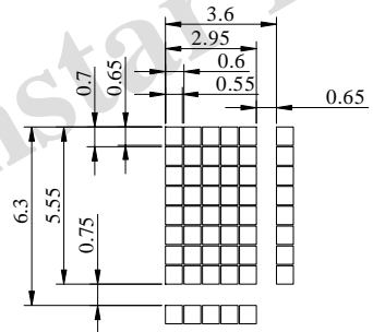
DOT SIZES SCALE 5/1
