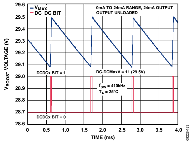
Figure 81. Operation on Reaching V_{MAX}
