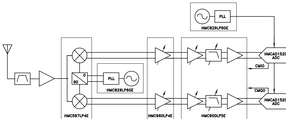
Figure 24. HMC829LP6GE in a typical receive chain
