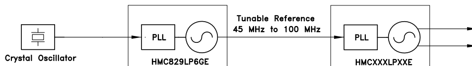
Figure 25. HMC829LP6GE used as a tunable reference for second HMC829LP6GE
