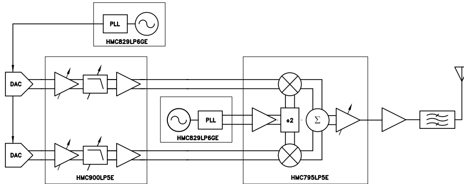
Figure 23. HMC829LP6GE in a typical transmit chain
