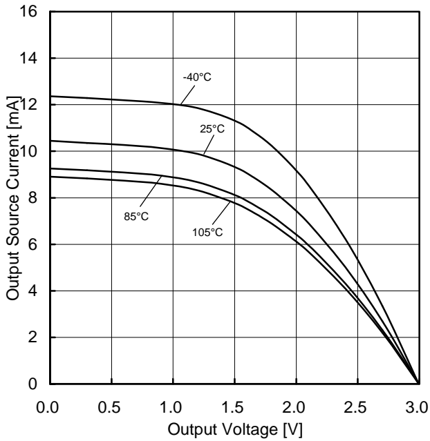
Figure 9. Output Source Current vs Output Voltage (VDD=3 V)
