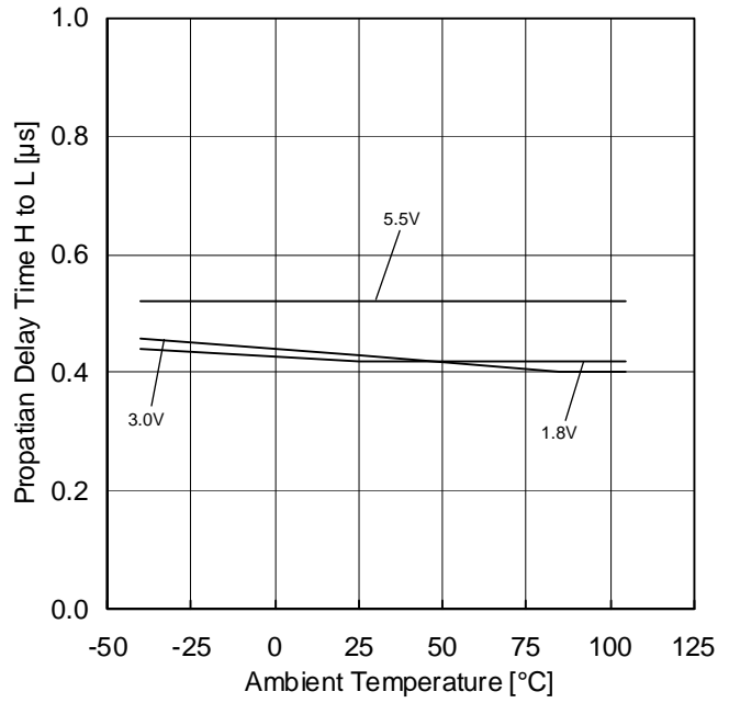
Figure 22. Propagation Delay Time H to L vs Ambient Temperature ( C_L=15\text{pF} , I_N=1.5\text{V} 100mV Overdrive)
