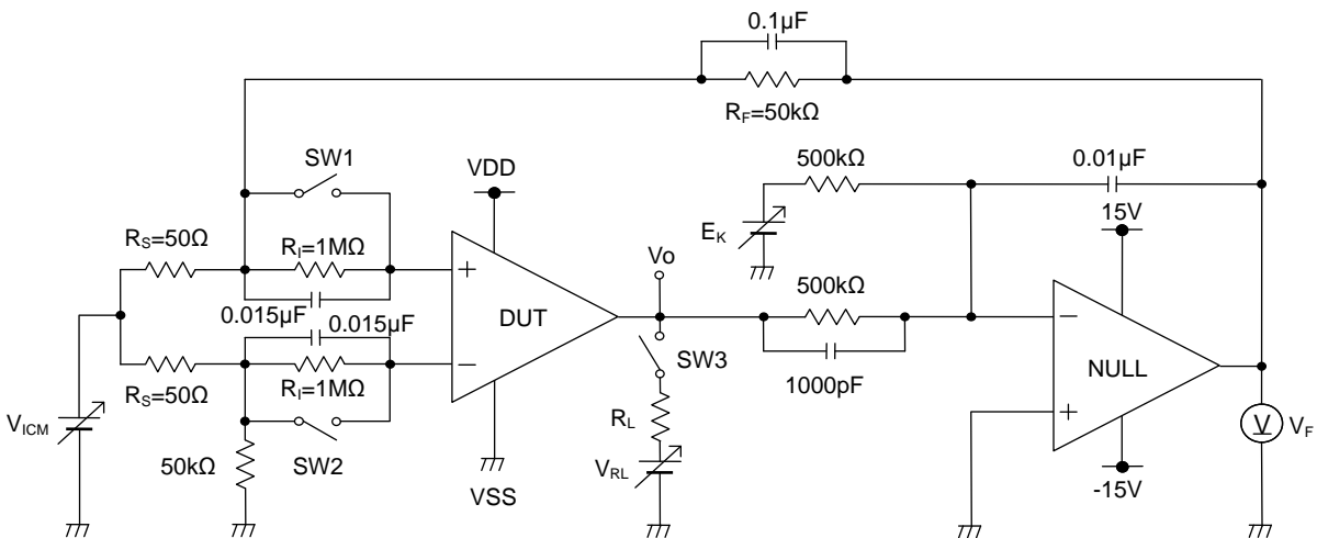
Figure 23. Test Circuit 1
