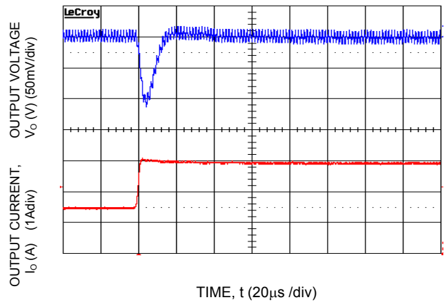
Figure 34. Transient Response to Dynamic Load Change from 50% to 100% at 12Vin, C_{out}=1x47\mu\text{F} , C_{Tune}=820\text{pF} & R_{Tune}=261
