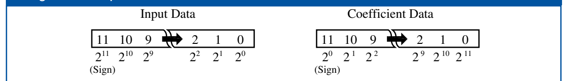
Figure 16. Input Formats
