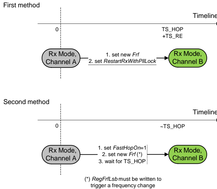
Figure 27. Receiver Hopping
