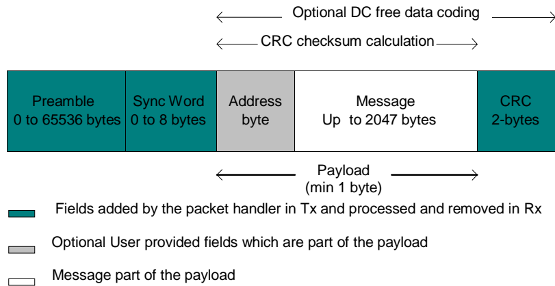
Figure 39. Fixed Length Packet Format
