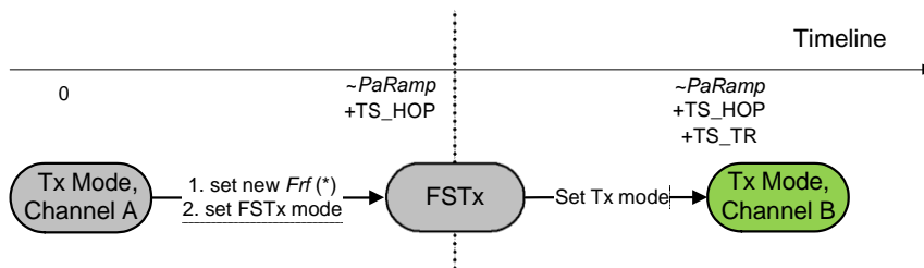
Figure 28. Transmitter Hopping
