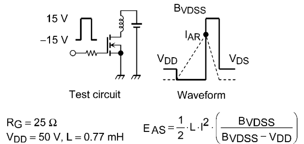
Fig. 8.16 Test Circuit/Waveform
