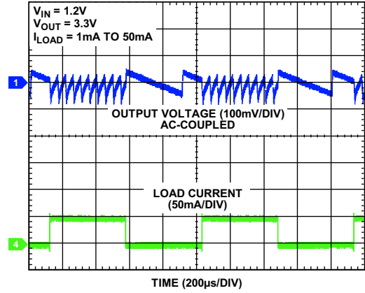
Figure 18. PFM Mode Load Transient Response (Auto Mode Part)
