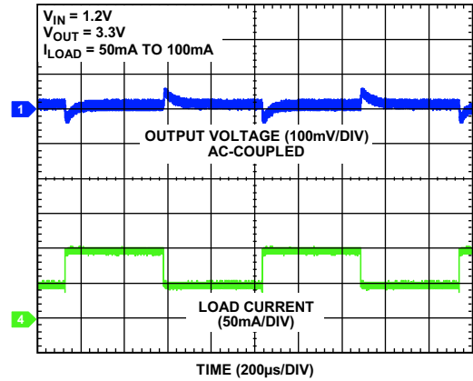
Figure 19. PWM Mode Load Transient Response (Fixed PWM Mode Part)
