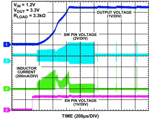
Figure 20. Startup, R_{LOAD} = 3.3\text{ k}\Omega
