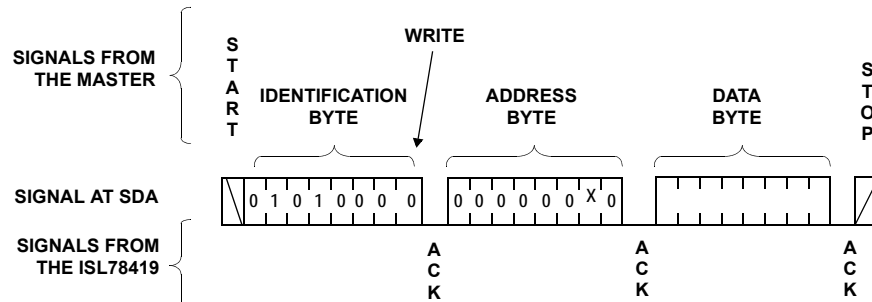
FIGURE 17. BYTE WRITE SEQUENCE
