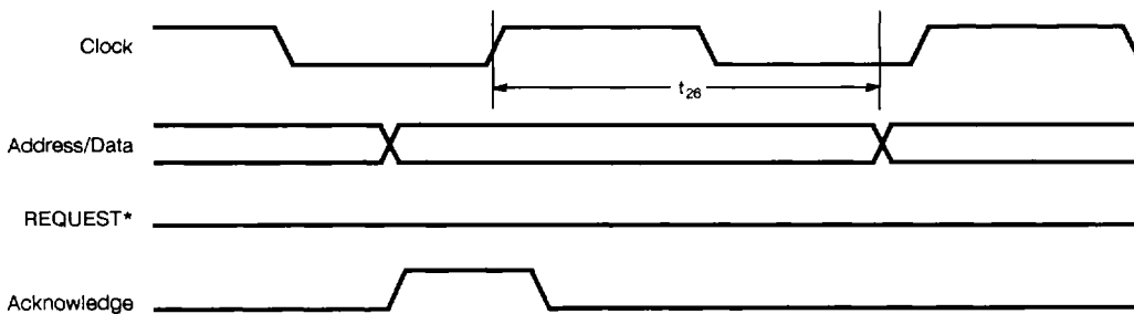
Figure 13. Address/Data Out
