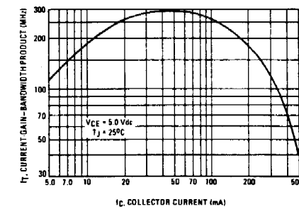
FIGURE 4 - CURRENT-GAIN-BANDWIDTH PRODUCT
