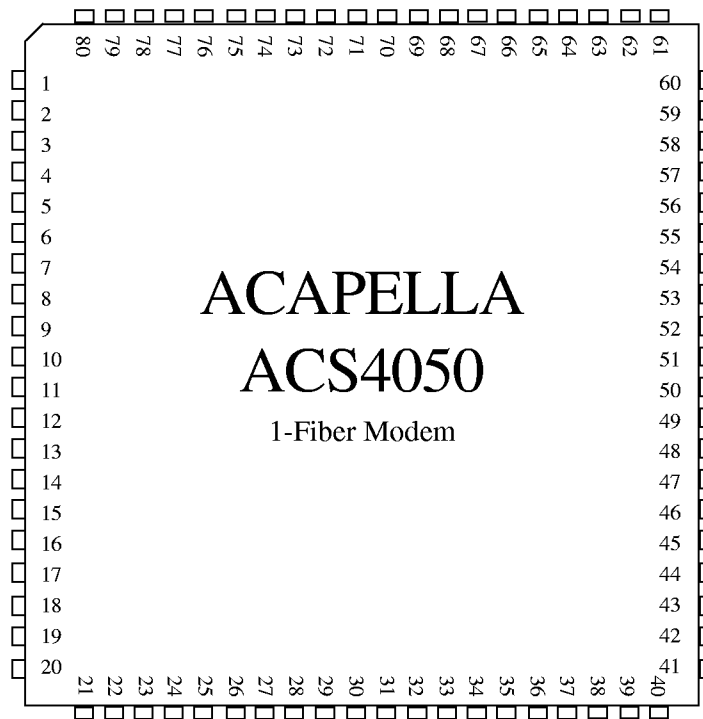
Figure 7. Top view of 80 pin TQFP package
