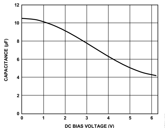
Figure 28. Typical Capacitor Performance
