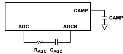
Figure 9. AGC Connections
