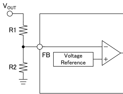
Figure 31. Feedback Resistor Circuit
