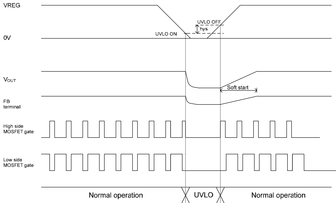
Figure 27. UVLO Timing Chart
