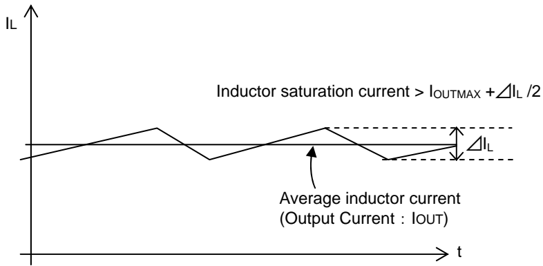
Figure 29. Waveform of current through inductor
