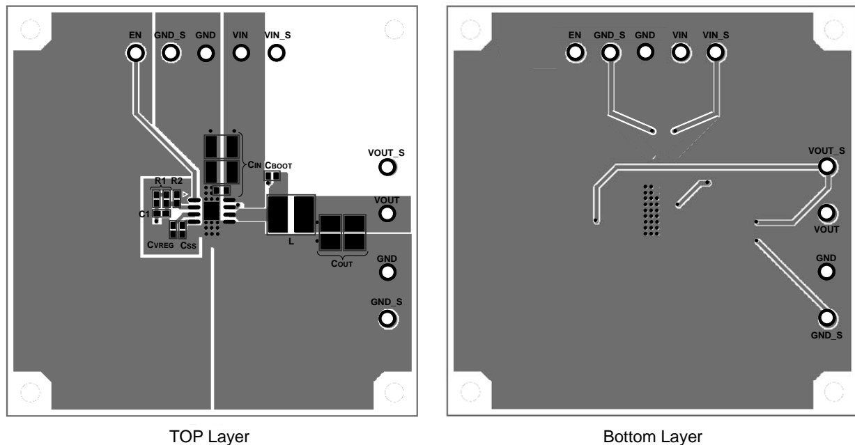
Figure 33. Example of PCB layout
