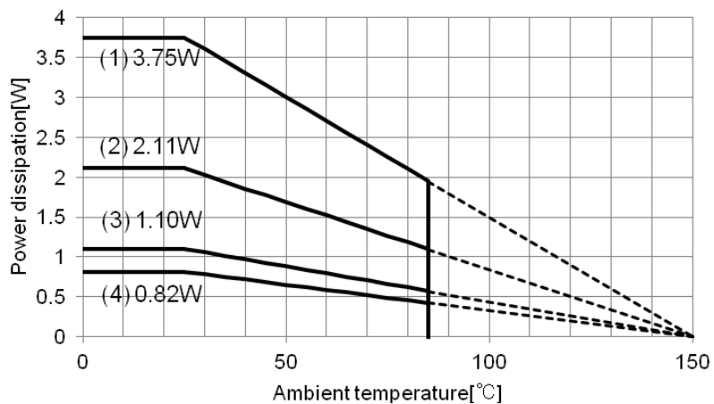
Figure 34. Power dissipation (HTSOP-J8)
