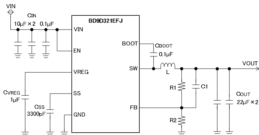
Figure 28. Application Circuit
