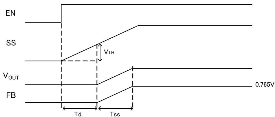
Figure 25. Soft Start Timing chart
