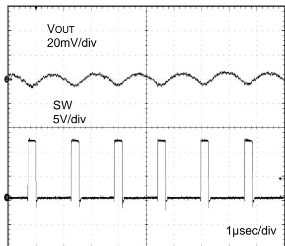
Figure 23. SW Waveform (② PWM control) ( V_{IN} = 12V , V_{OUT} = 1.8V , I_{OUT} = 3A )
