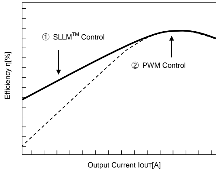
Figure 21. Efficiency (SLLM™ Control and PWM Control)
