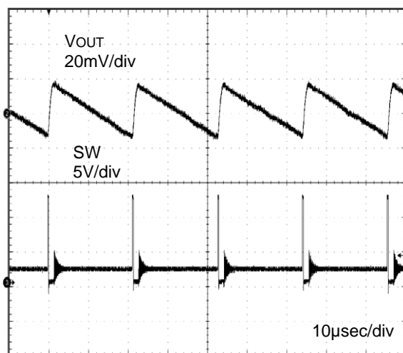
Figure 22. SW Waveform (① SLLM™ control) ( V_{IN} = 12V , V_{OUT} = 1.8V , I_{OUT} = 30mA )
