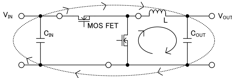
Figure 32. Current Loop of Buck Converter
