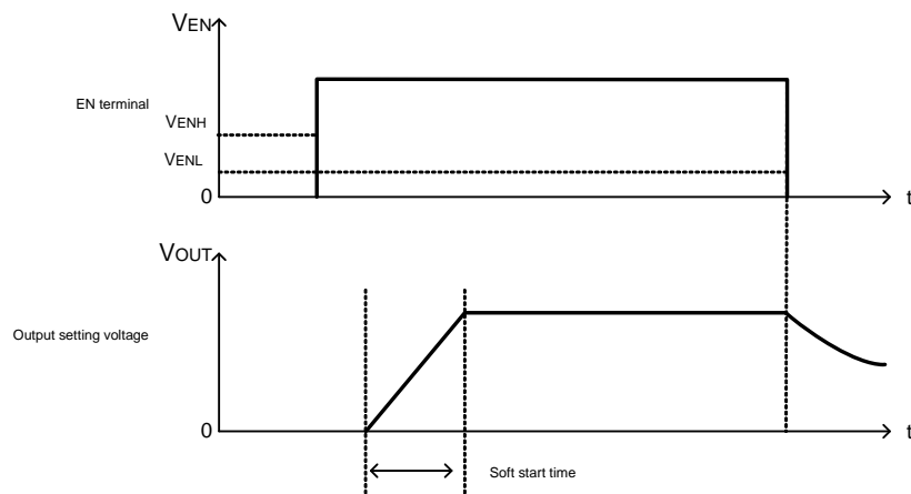
Figure 24. Start-up with EN pin
