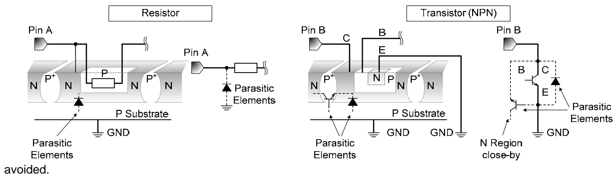
Figure 36. Example of monolithic IC structure
