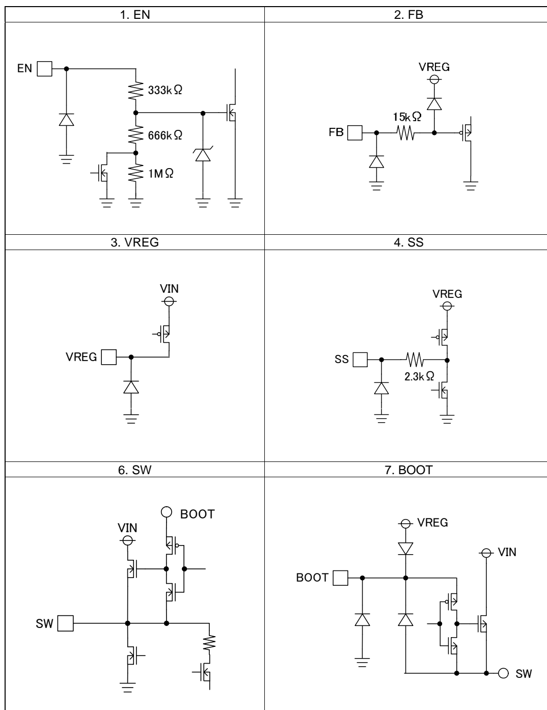
Figure 35. I/O equivalence circuit
