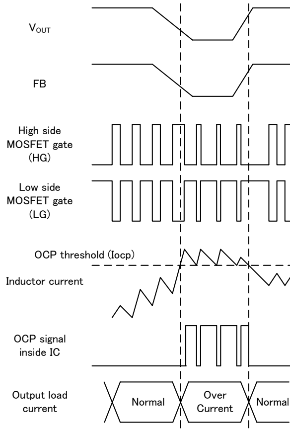
Figure 26. Over current protection timing chart
