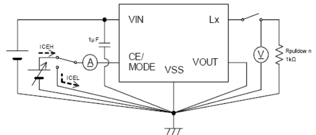
Circuit ⑧
