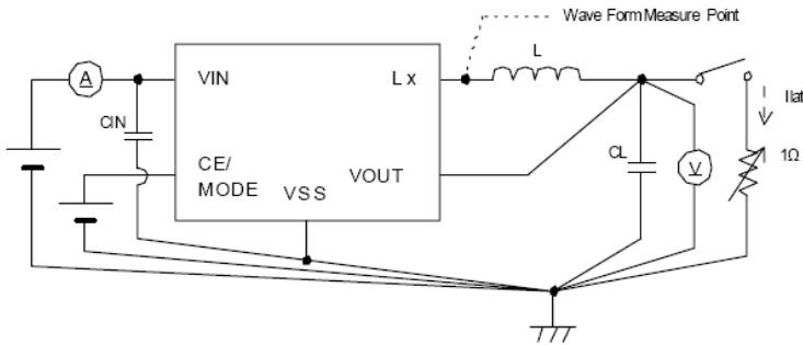
Circuit ⑨
