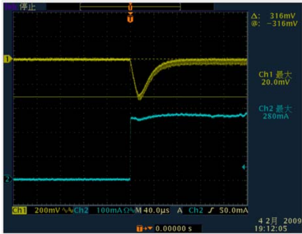
VIN=5V,IOUT=0~300mA
