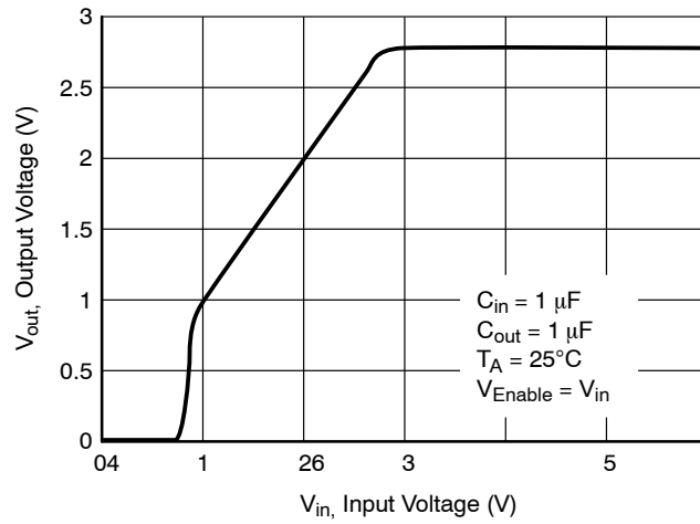
Figure 25. Output Voltage vs. Input Voltage
