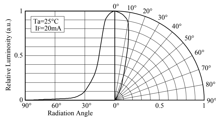
■ Directivity (NSPB510(S))
