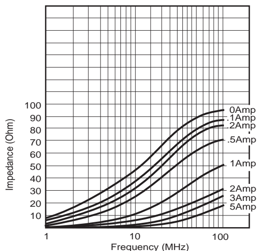
IMPEDANCE VS. DC BIAS SMB30 & SMB40
