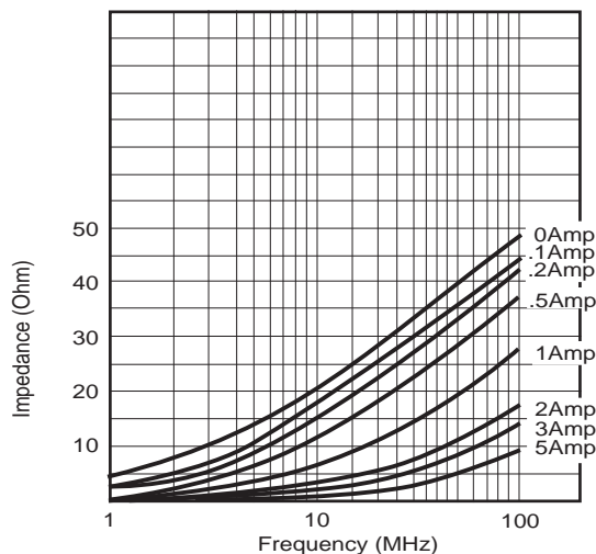
IMPEDANCE VS. DC BIAS SMB20
