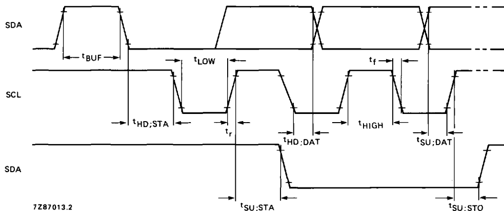
Fig. 11 Timing.
