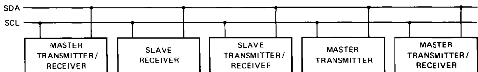
Fig. 9 System configuration.
