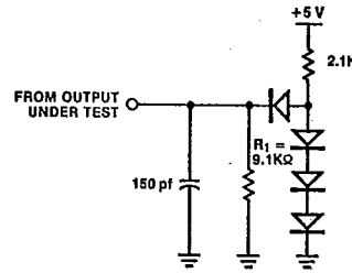
Figure 19. Test Load 1
