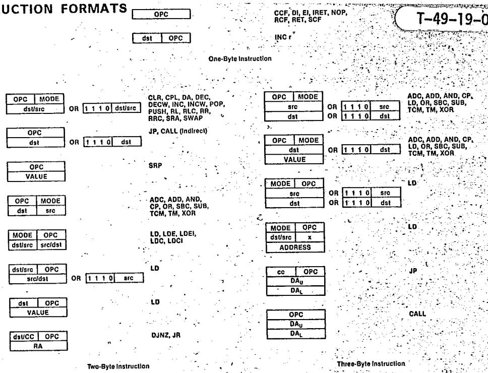
Figure 17. Instruction Formats
