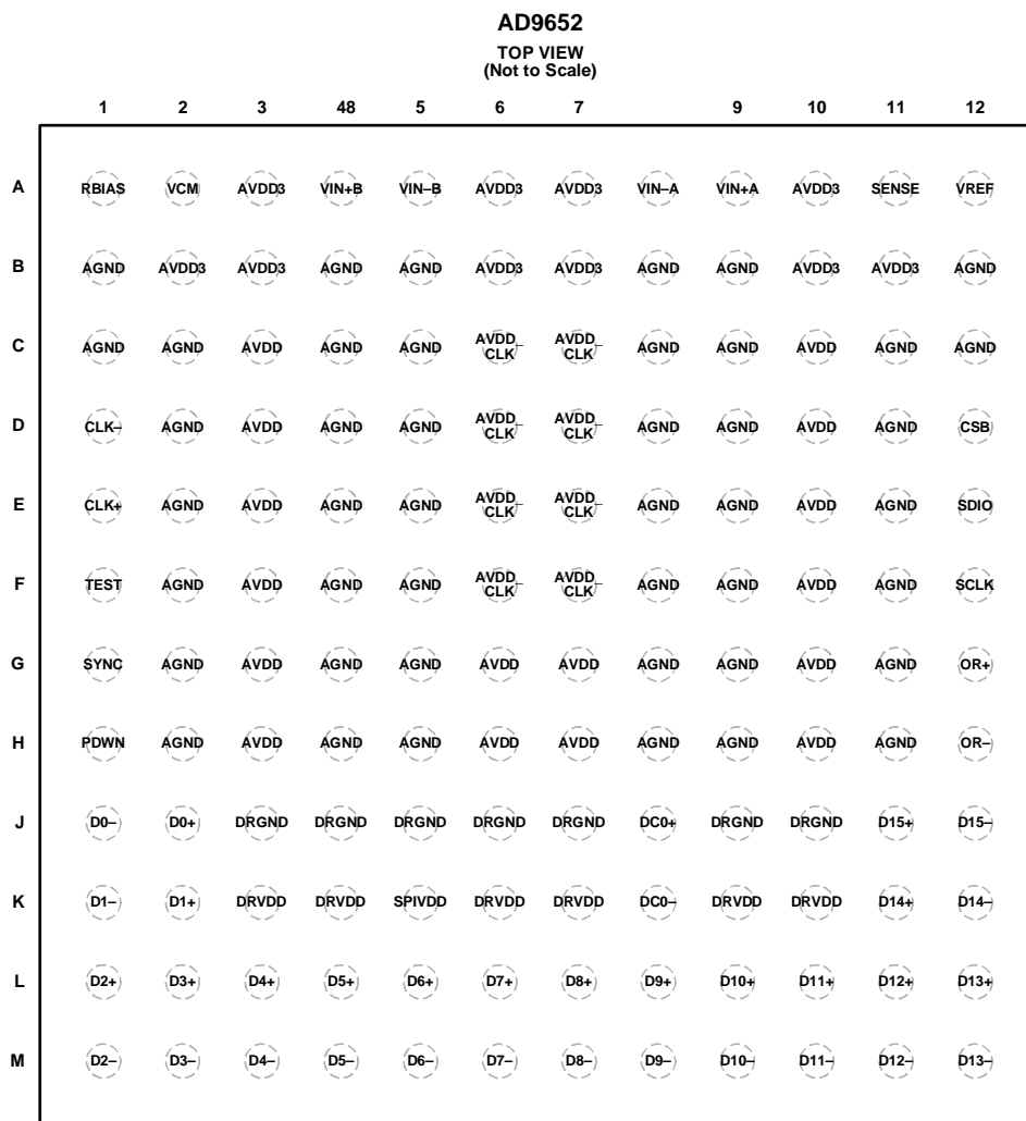
Figure 5. Pin Configuration
