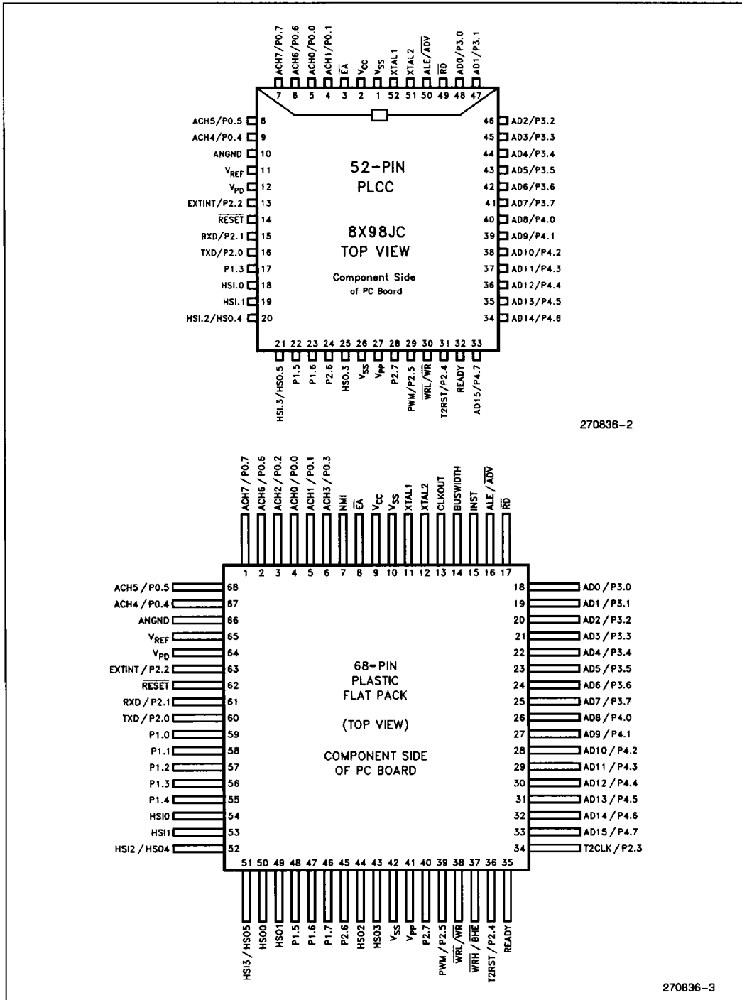
Figure 4. Package Diagrams
