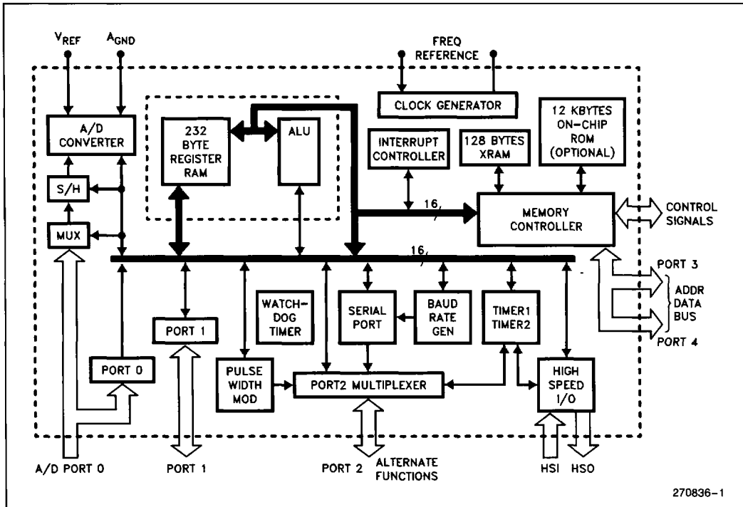
Figure 1. 8X9XJC Block Diagram
