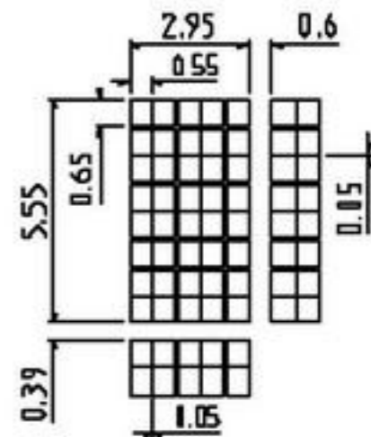
A BLOCK
