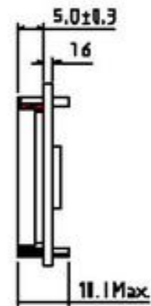
REF,EL,B/L
