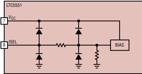
Figure 15. ISEL Interface Schematic
