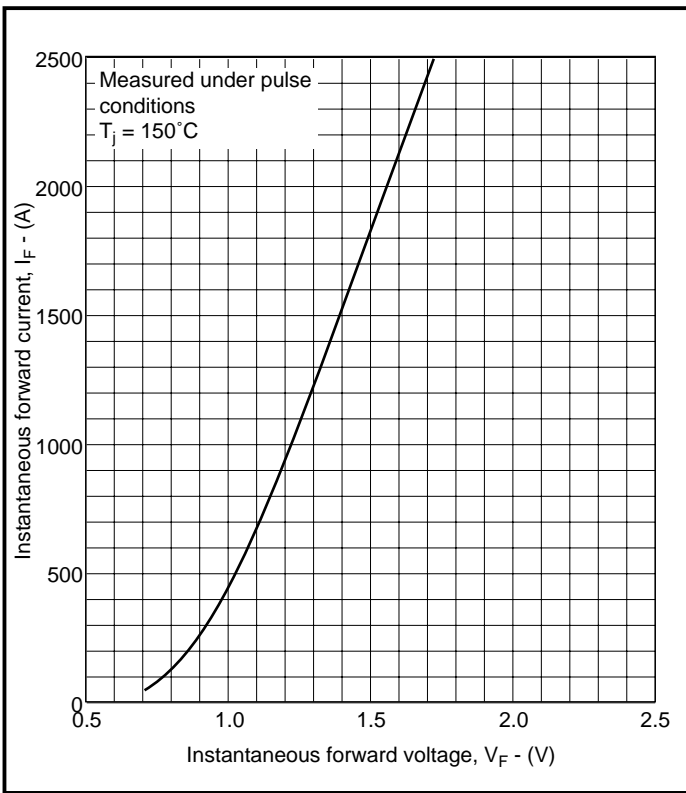
Fig. 3 Maximum (limit) forward characteristics
