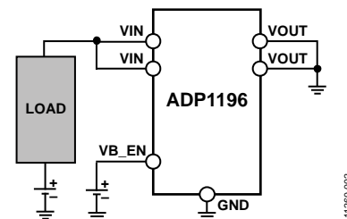
Figure 2. High-Side Load Application
