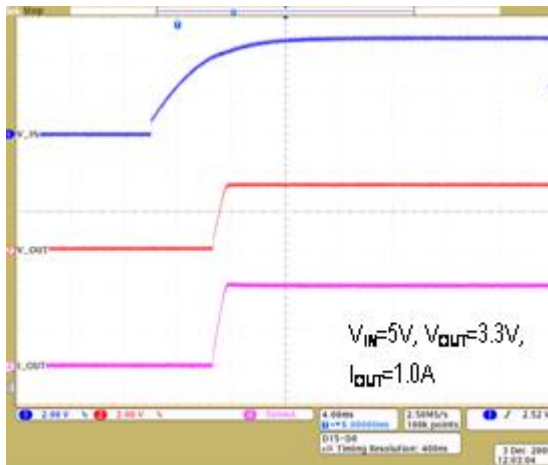
Power-on Waveform
