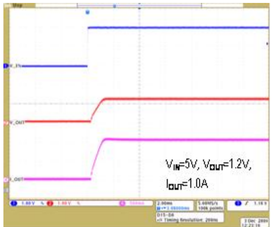
EN-ON Waveform
