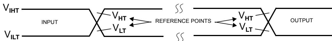
Figure 10. AC Input and Output Reference Waveforms
