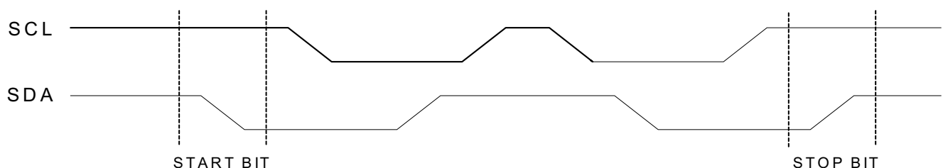
Figure 2. Start/Stop Definition
