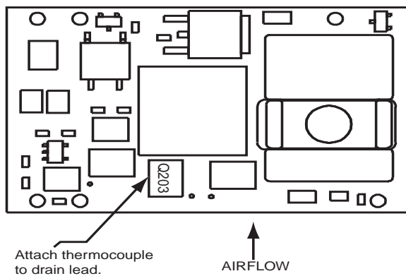
Figure 43. HW/HC 6.6A-12A-Series Temperature Measurement Location (Top View).
