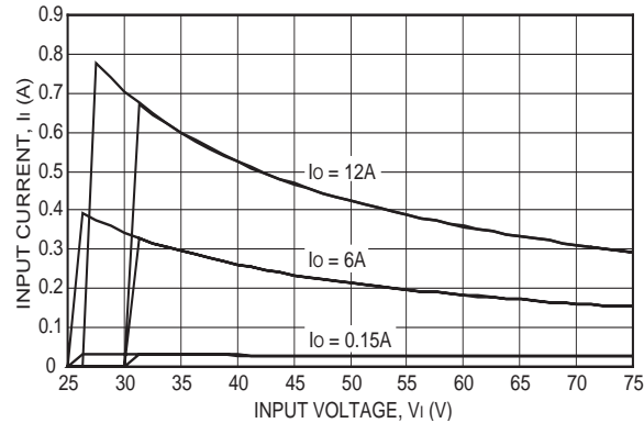
Figure 7. Input Voltage and Current Characteristics.
