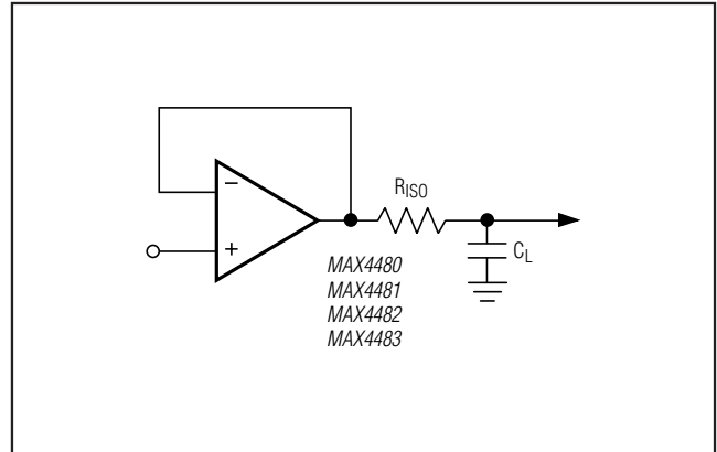
Figure 3. Capacitive-Load-Driving Circuit
