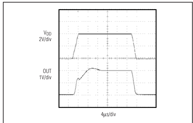
Figure 5. Power-Up/Down Waveform
