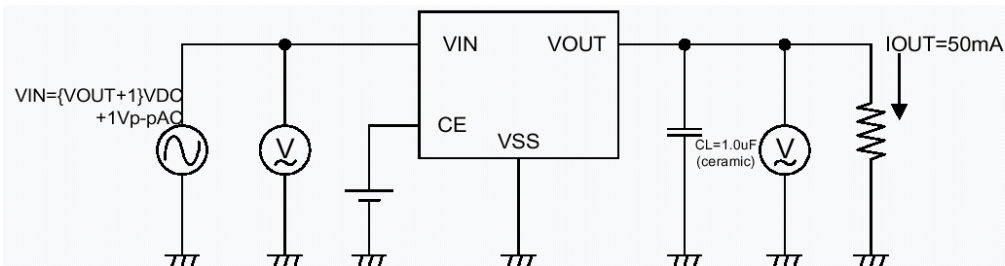
Circuit 4
