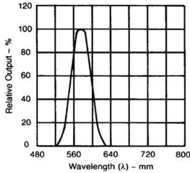
Fig. 2. Spectral Response
