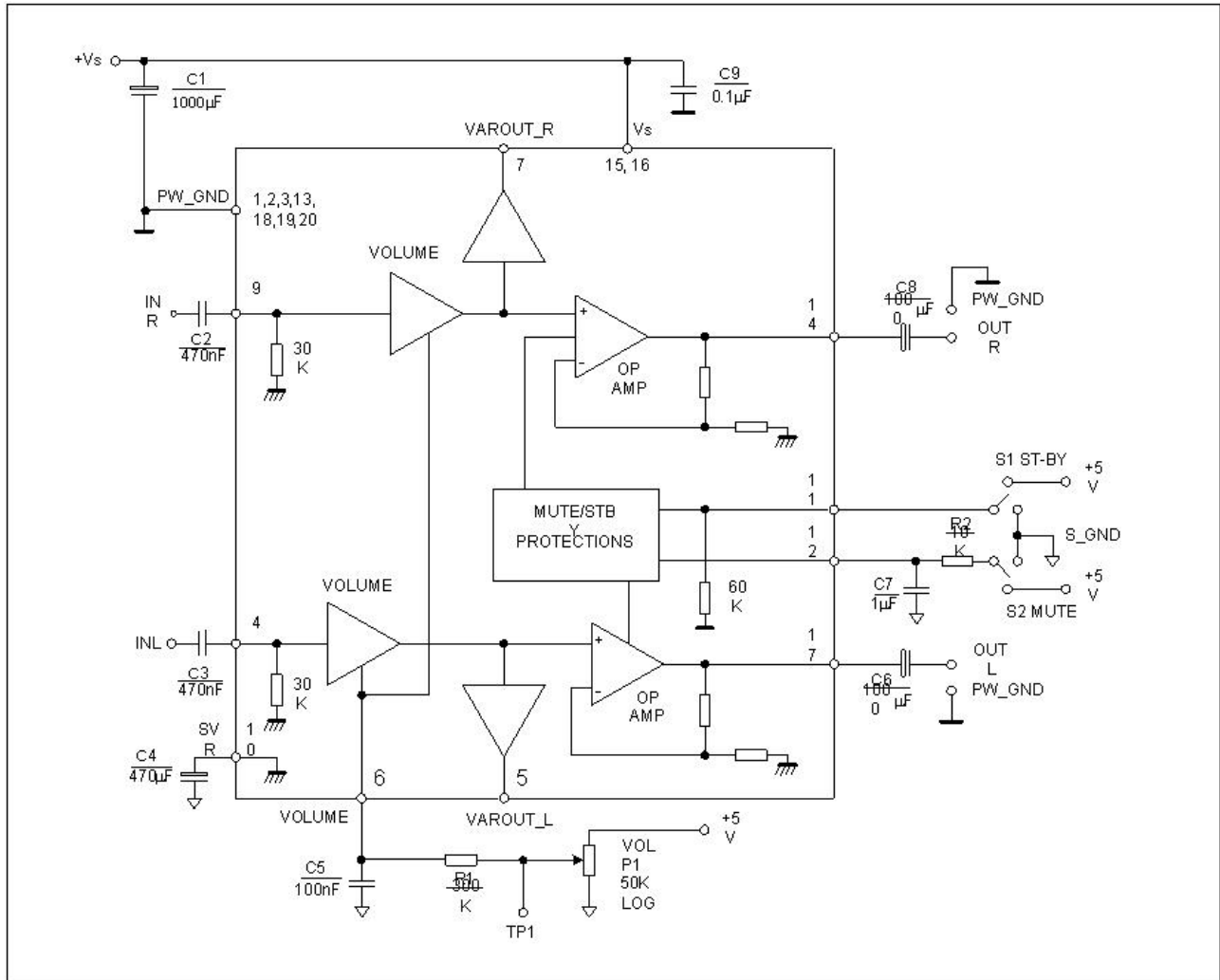
Figure 1A. Application Circuit
