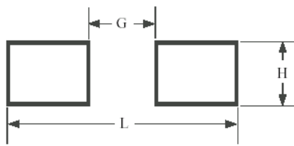
Fig. 2 Solder pads scheme and recommended dimensions.
