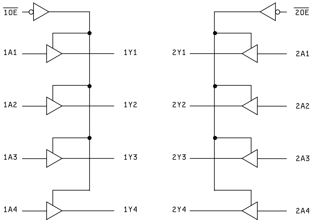
FIGURE 4. Logic diagram.
