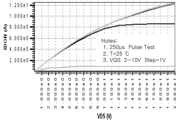
Fig. 1. On-state characteristics
